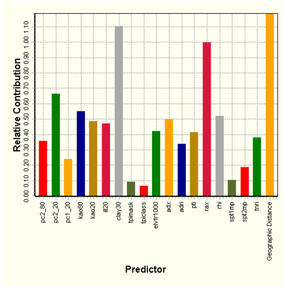
Figure 29. Relative contribution of predictors in the GDM model. Labels are defined in (Table 18)
